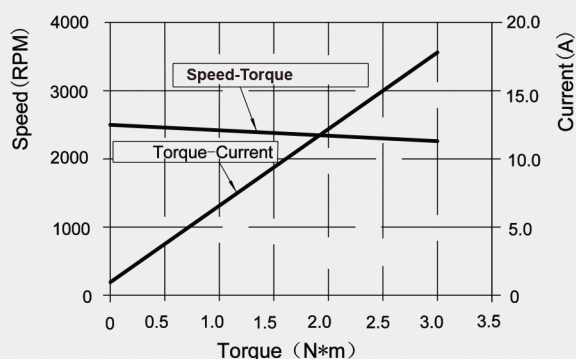
Torque-Speed- Current
